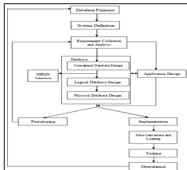
Gambar 1. Tahapan DBLC
