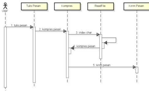
Gambar 17 Sequence Diagram Kirim Pesan
