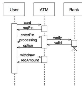
Gambar 9 Contoh Sequence Diagram
