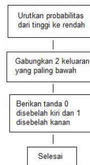
Gambar 2 Alur Kode Huffman
