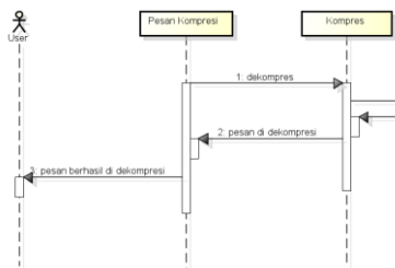
Gambar 18 Sequence Diagram Dekompresi Pesan
