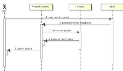
Gambar 19 Sequence Diagram Baca Pesan
