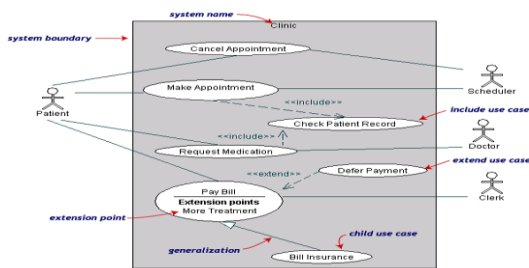
Gambar 7 Contoh Use Case Diagram
